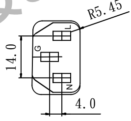
IEC-60320-C13
